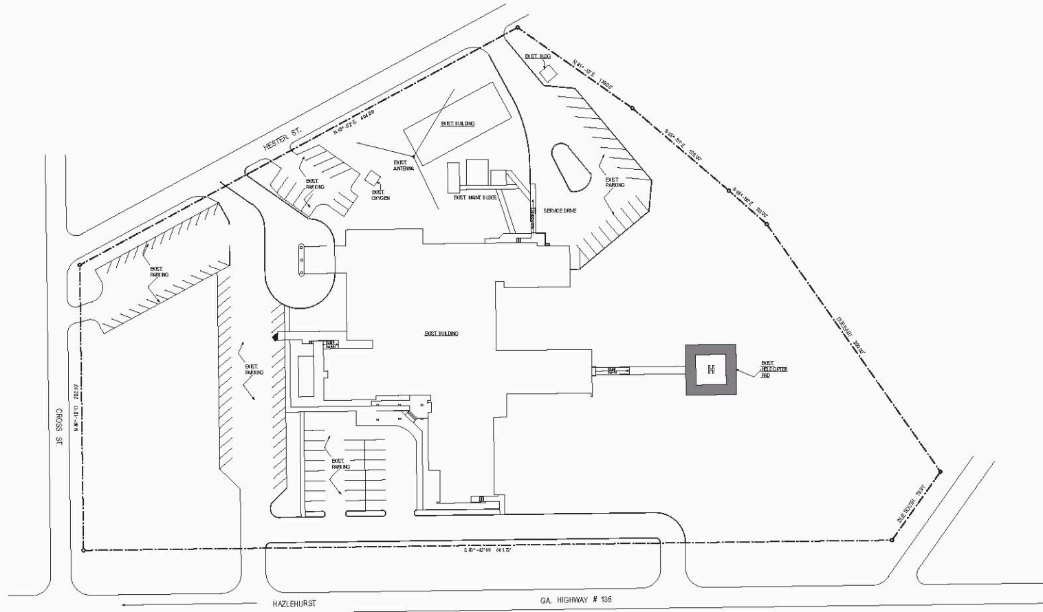
SITE PLAN 1" = 40'-0"
